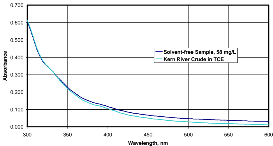
Figure 11. Kern River crude oil spectra.
