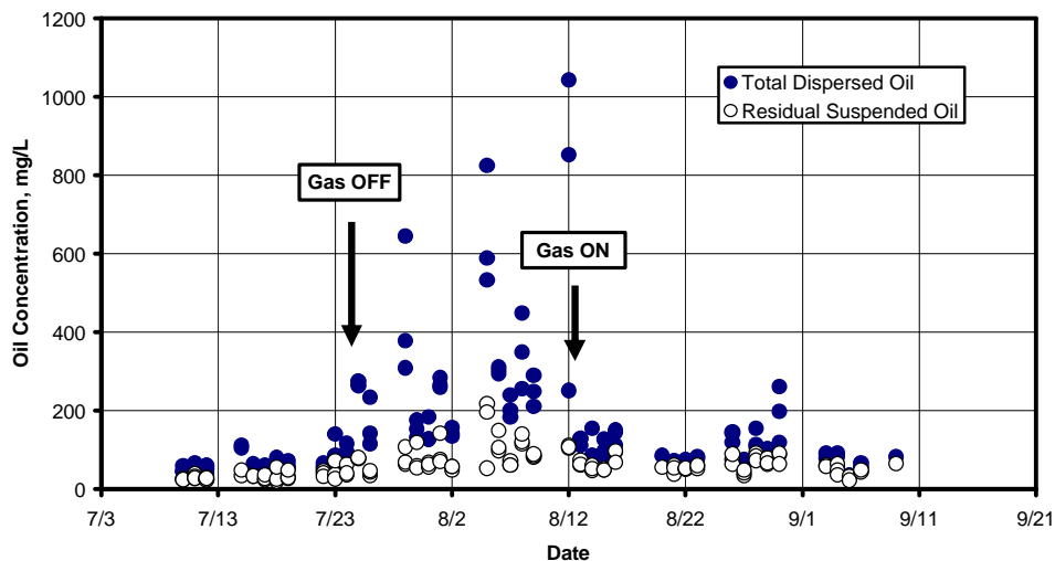
Figure 12. Effect of educted gas on oil content at effluent of Surge 2.
