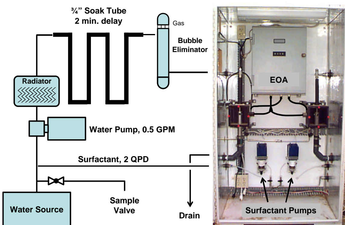
Figure 4. Typical EOA installation.
