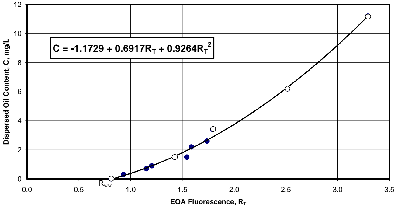
Figure 5. EOA calibration curve – FC-5, produced water.
