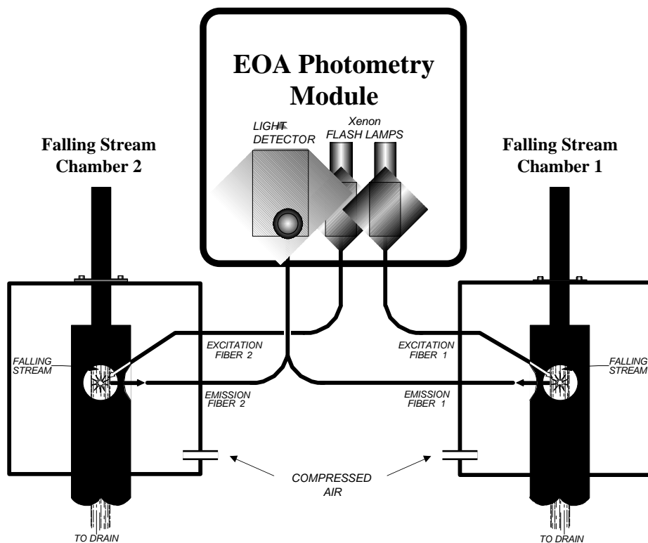
Figure 2. Schematic diagram of the EOA System.
