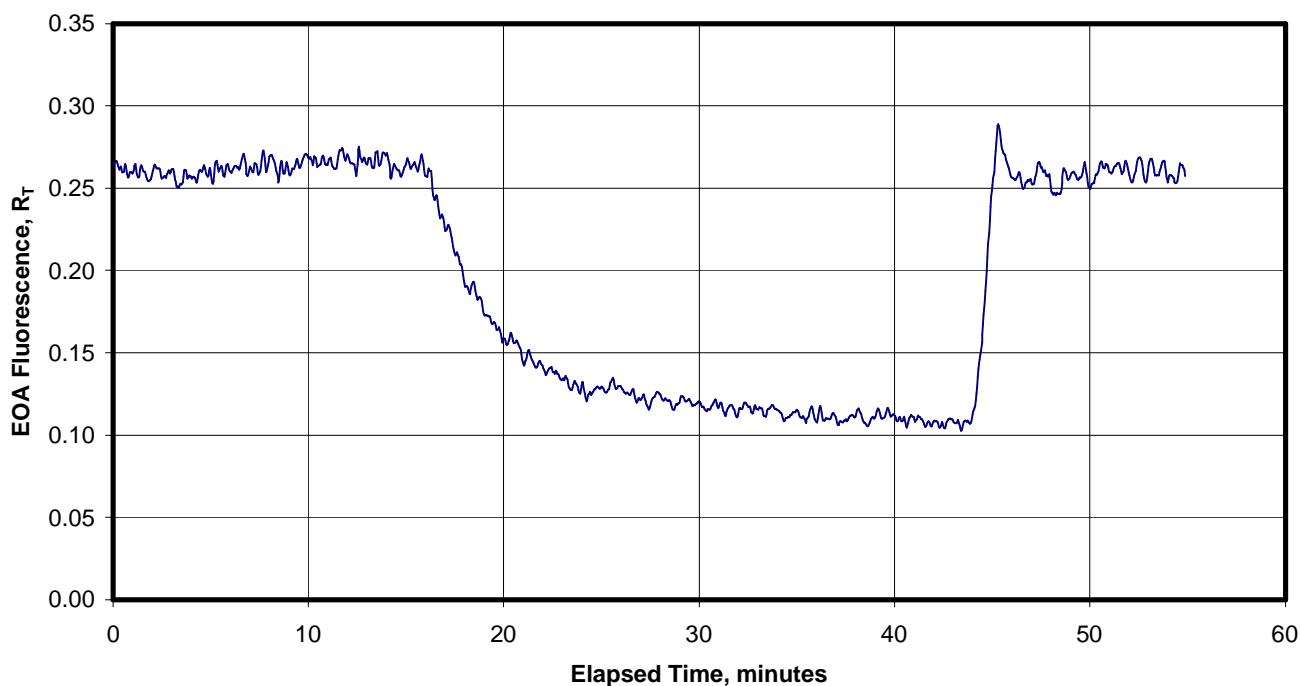
Figure 3. Effect of surfactant addition on dispersed oil fluorescence.
