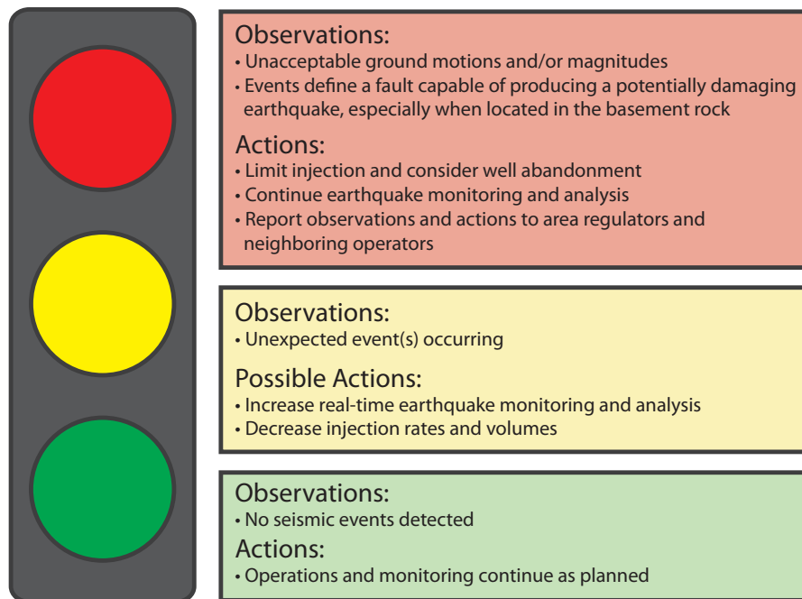
Figure 5. Traffic light system applicable to saltwater disposal. The green, amber, and red panels represent the levels of heightened awareness frequently represented in traffic light systems. Within each panel we suggest what observations might be considered and possible actions to take.
